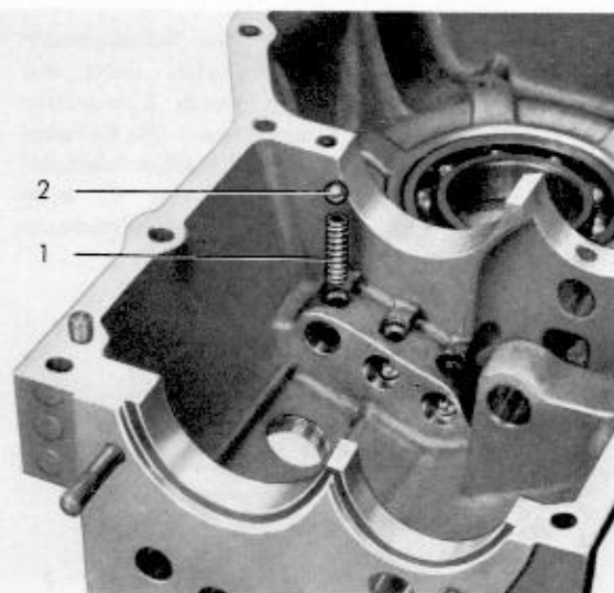
1 - Feder
